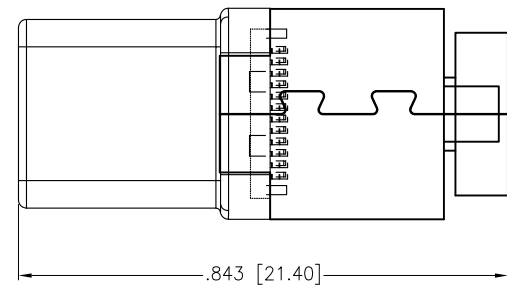
ASSEMBLY
