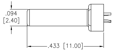
CONNECTOR
