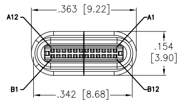
CONNECTOR
