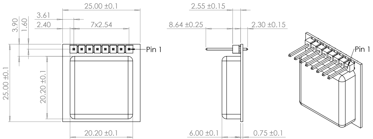
Figure 14: Outline dimensions K-LD2
