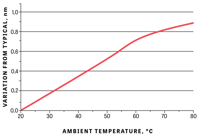
WAVELENGTH SHIFT WITH TEMPERATURE
