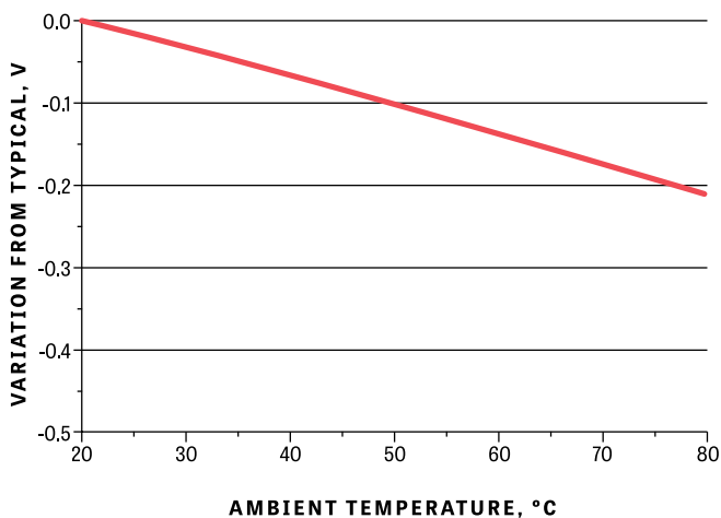
VOLTAGE SHIFT WITH TEMPERATURE
