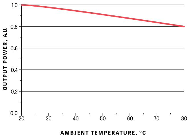
OUTPUT POWER OVER TEMPERATURE
